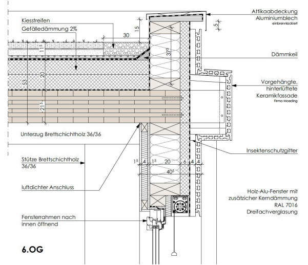
DETAIL ATIKA | M 1:10
